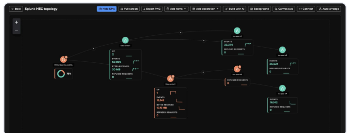
Splunk HEC: the live topology of pools and endpoints, availability, events and the member that stopped.
