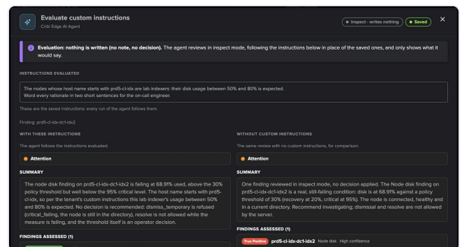
Custom instructions, evaluated: the same finding reviewed with and without them, writing nothing.
