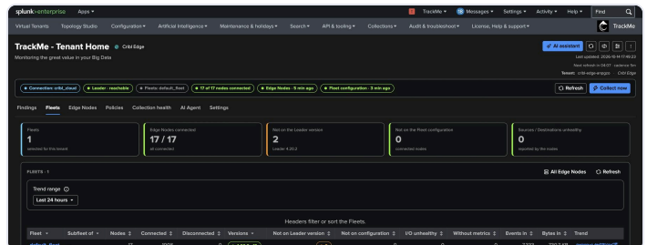
Cribl Edge: the Fleet at a glance, 17 of 17 nodes connected, versions and the 24-hour trend.
